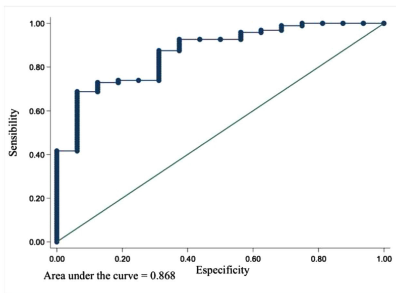
Figure 1 ROC and AUC for prognostic model 1 (INR/ALT).
