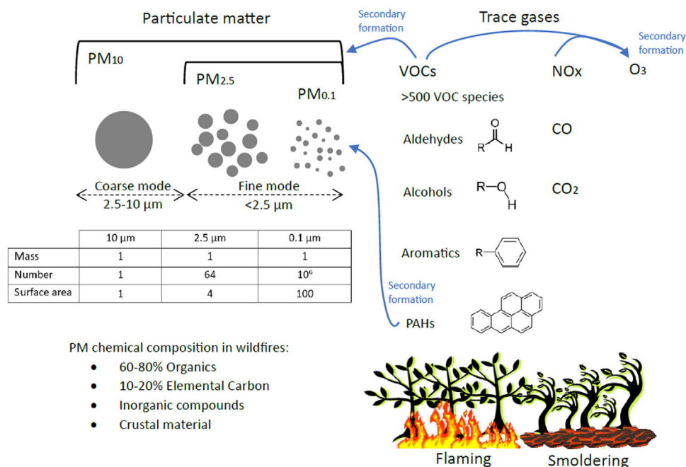
Figure 2 WFS contains a myriad of air pollutants, including particulate matter and trace gases. Photochemical reactions lead to the formation of secondary pollutants like O 3 and secondary organic PM. The insert table compares the physical properties of three samples of PM with the same mass concentration (arbitrarily defined as 1) but with different particle sizes. Fine mode particles have higher number concentrations and surface area compared to coarse mode particles. The ability of PM 2.5 and PM 0.1 to penetrate deeper into the respiratory system and their higher surface area result in higher toxicity compared to larger particles.
